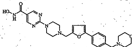
compound 9 .047 H 2 O .1.99 CF 3 COOH
